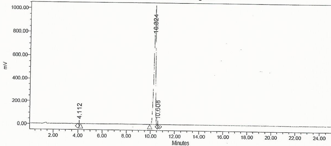
Auto-Scaled Chromatogram
